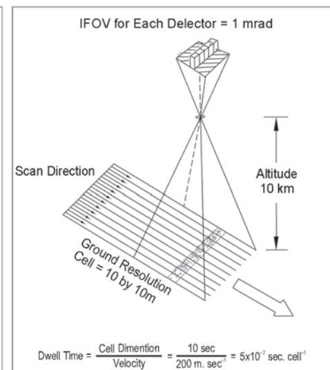
6.8 Pushbroom Scanners
