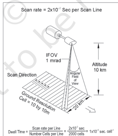
6.7 Whiskbroom Scanners
