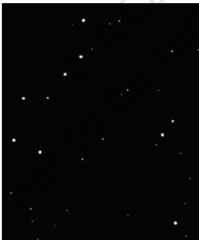
Fig. 12.2: A part of the night sky
