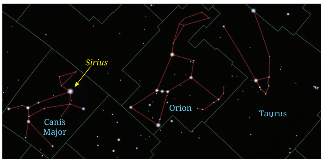
Fig. 12.3: Some constellations and stars
