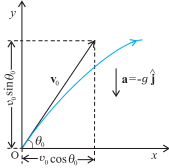
Fig 3.16 Motion of an object projected with velocity v_o at angle \theta_o .
